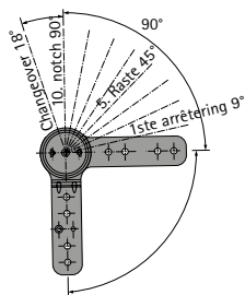
FrankoFlex Basic position 90°
